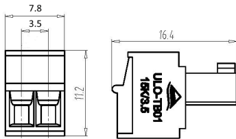
Power plug
